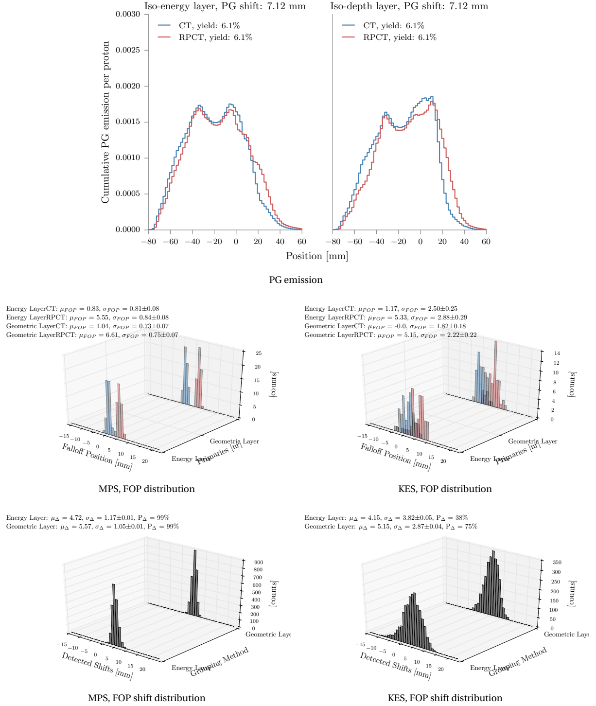
Figure 20: On top the PG emission profile (along the beam) is shown: left the iso-energy and right the iso-depth spot groupings, again in blue the CT and red the RPCT. On the second row, we see the FOP distributions with on the left the MPS and the right the KES results. The bottom row shows the FOP shift distributions.
