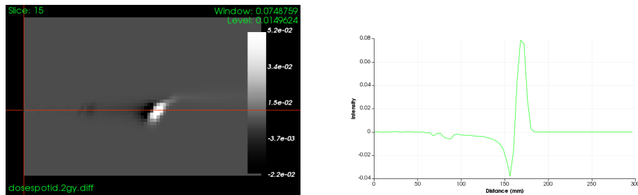
Axial slice of the absolute dose difference for spot 61 of our TP; color scale chosen for best visibility. A relatively uniform forward shift may be observed.
