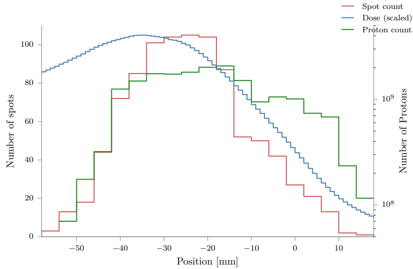
Figure 13: For the main field in the TP, per spot, a FOP is computed and binned (red, left y-axis). The depth dose distribution is overlaid in blue in linear arbitrary scale, as a reference for the shape. In green each spot is weighted with its number of protons (right y-axis) and then summed. With respect to the red line, the green line flattens out the top in the forward direction, supporting the thesis that in the geometric domain as well as the energy domain, the distal spots are individually weightier. However the cumulation of all spots leads to a larger dose in the medial layers of the target volume.
