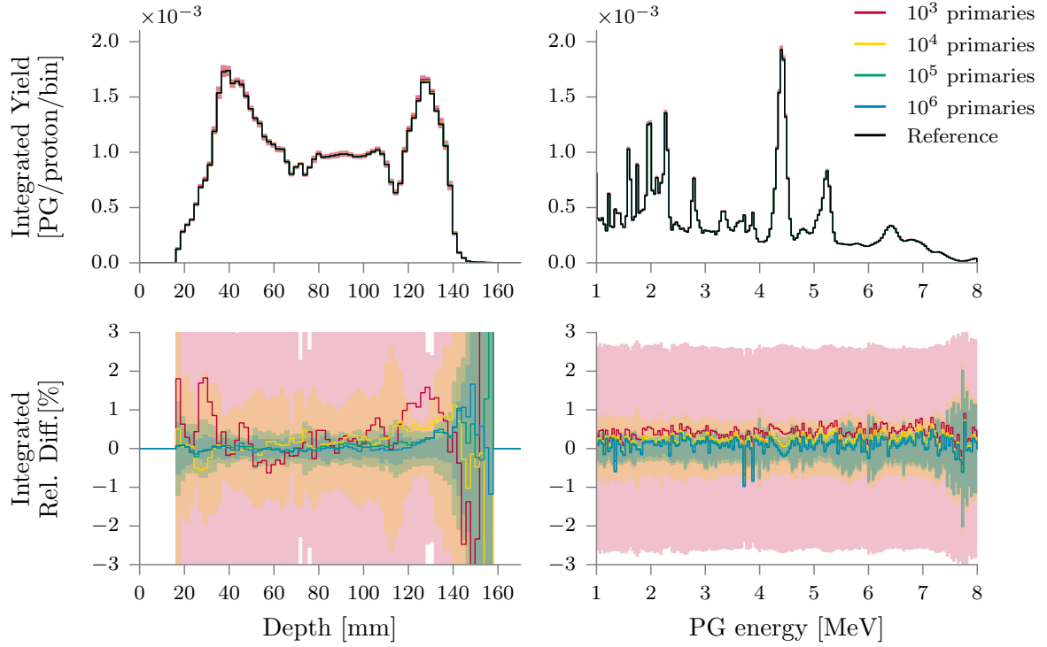
Figure 7: Test case 2. Row 1 shows the PG yields and row 2 the relative difference with respect to the reference ( \frac{vpgTLE-Reference}{Reference} ). For both rows, note that the yield was integrated over all other dimensions. The left column is a projection along the beam-axis, while the right column shows the spectral bins integrated over all voxels considered. The shaded areas represent 2\sigma error bands, where \sigma is the standard deviation over the mean of 10 simulations.
