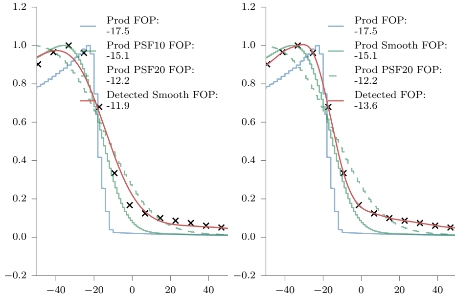
Figure 5.2: On the left and right the PG production (Prod) is given in blue, that signal convoluted with a Point Spread Function (PSF) with smoothing parameter 10 mm and 20 mm (dashed) in green, and the detected response in black crosses. Red are the fitted curves, on the left with \lambda = 2 and on the right \lambda = 0 . The cost of smoothing, required especially for lower statistics, comes at the price of a FOP shift.
