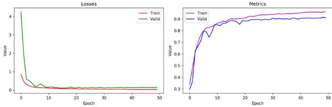
FIGURE 7.12: Training curves of a reduced U-Net trained on 200 patients and validated on 100 with a categorical cross-entropy loss and the Adam optimizer with a learning rate of 2 \times 10^{-3} . Dice results are given on the right. [122].
