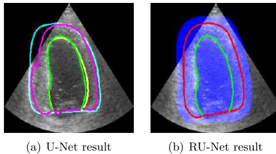
FIGURE G.1: Illustration of the refinement in place in RU-Net. The ROI is shown in blue. The ground truth is shown in yellow and cyan while the prediction is on green and red/magenta. On the U-Net epicardium contour (magenta), we see the epicardium being locally discontinuous while it is not the case for RU-Net (red).
