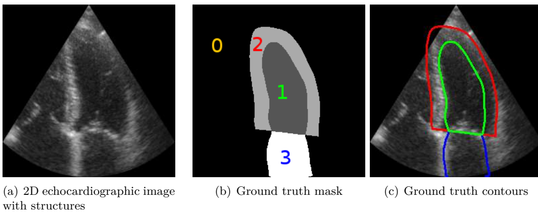
FIGURE 4.3: Multi-structure segmentation seen as a multi-label classification problem. Supervised learning algorithms are trained to predict b) from a). In visuals, we traditionally display the contours over the image as in c).
