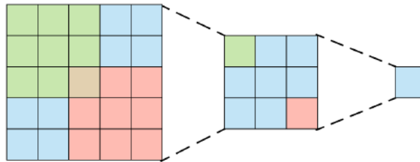
FIGURE 7.6: Receptive fields [123]: After 2 \times 3 \times 3 convolutions, the pixel on the right contains global information about the 5 \times 5 region on the left. As CNNs get deeper, the receptive field increases, allowing to extract high-level features.
