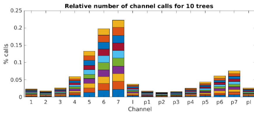
FIGURE 6.9: Relative number of calls for 7 scales of features on ten mid-size trees ( 5 \times 10^4 patches). Regular features on the left, pairwise on the right.
