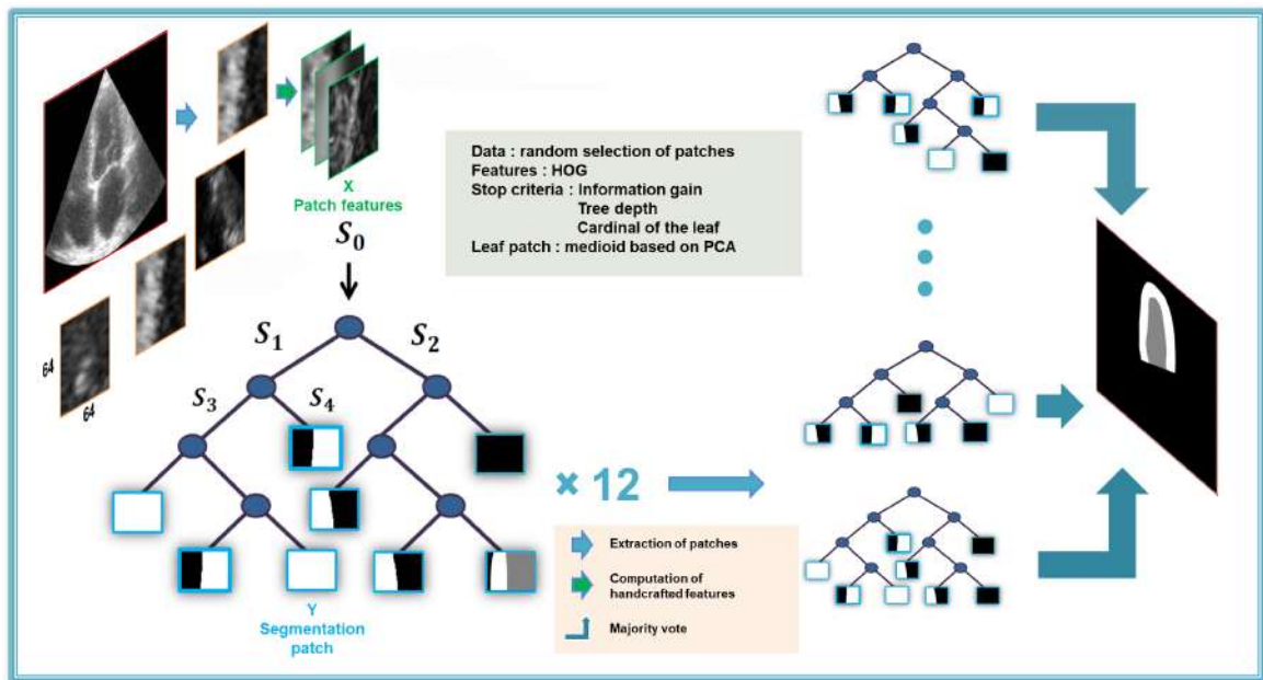
FIGURE 6.12: Our SRF summary [31]
