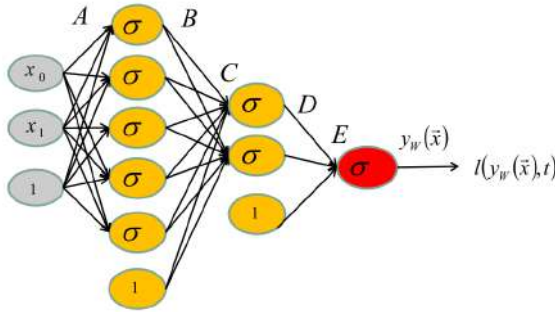
(a) Backpropagation illustration on a fully connected neural network [36]
