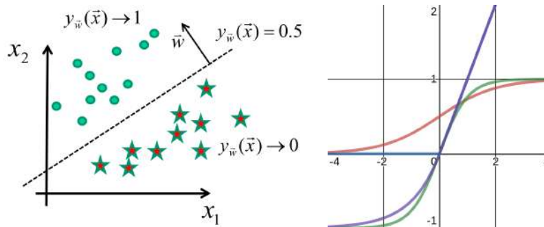
(a) Linear separation. The sigmoid has a similar behavior, except values close to 0 are linearly shifted while points far from the decision frontier tend towards 0 or 1 rather than being set to either. [36]
