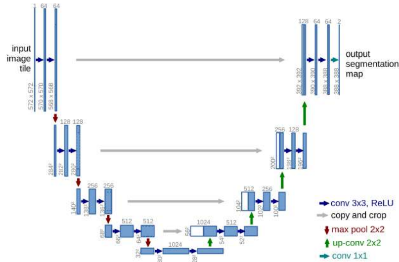
FIGURE 7.4: Representation of the layers and feature kernels of the U-Net [34]
