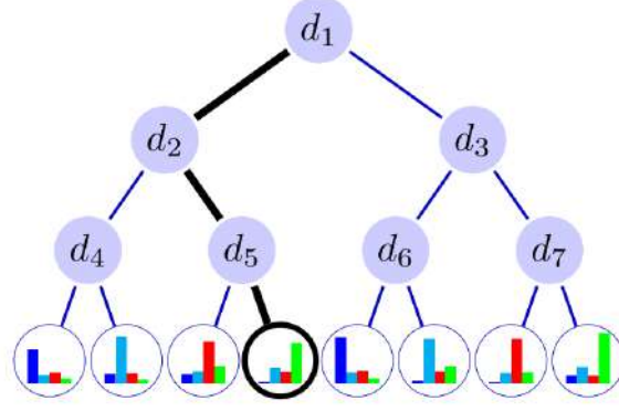
FIGURE 6.4: Tree representation: The information stored at the leaves after the training (here the histogram of labels) can be used at test time to assign a new class to the new data routed down to the leaf [108].
