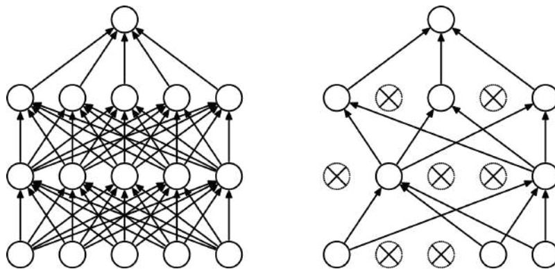
FIGURE 7.11: Dropout illustration [130]. Left: base network, right: network with a dropout rate around 40%.
