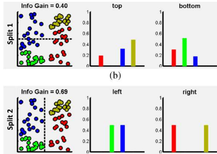
FIGURE 6.3: Stump illustration and resulting information gain [62]. The stump function is dotted. RFs perform linear cuts in the representation space.
