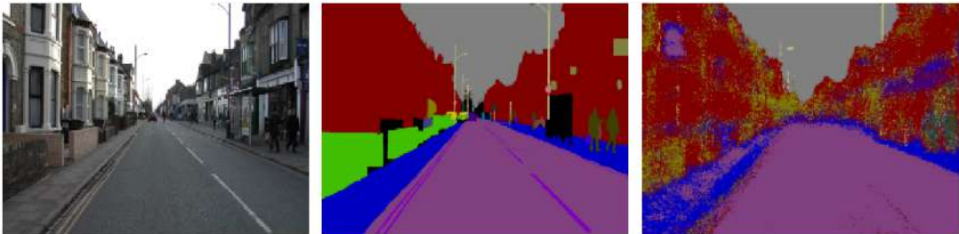
FIGURE 6.5: (left) Street view, (middle) its corresponding segmentation masks, (right) the prediction obtained from using RFs. [28].
