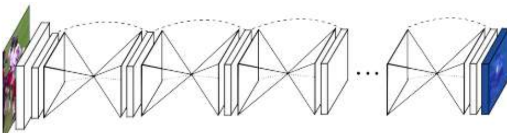
FIGURE 8.2: Original architecture of SHG. The input of cascaded networks is the concatenation of the original image and the previous segmentation result.
