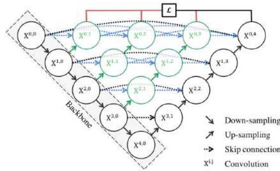
FIGURE 8.1: Original architecture of U-Net++. Deep supervision in red shows that a same loss L sends gradients to early reconstructions of the final segmentation in X^{0,4} . Additional convolutional layers on the skip connections are shown in green.
