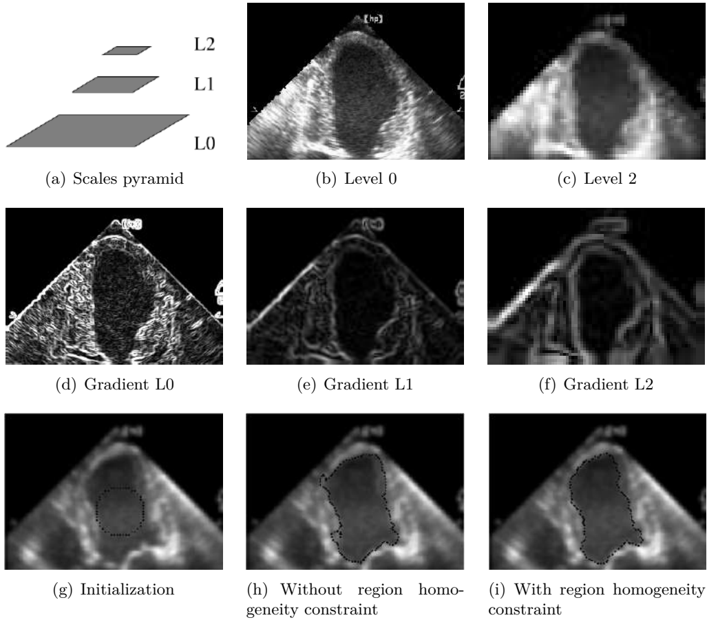
FIGURE 4.5: Illustrations from the level-set approach from (Ning et al., 2002) [77]. First rows: Multi-scale data-terms obtained by applying edge detection on the blurred downsampled image. Last row: Examples of segmentation results.
