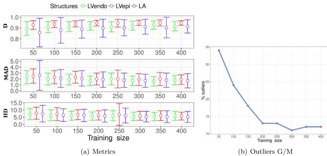
FIGURE 7.30: Evolution of the segmentation scores of U-Net 1 computed on fold 5 according to the number of patients in the training dataset
