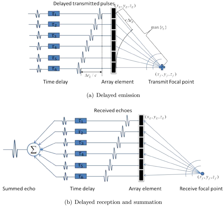
FIGURE 3.4: Focused beam onto a focal point. a: Each element receives a different delay according to the distance to the point. b: The same delays are applied on the received echoes before summation to create the radiofrequency (RF) echo signal [58].
