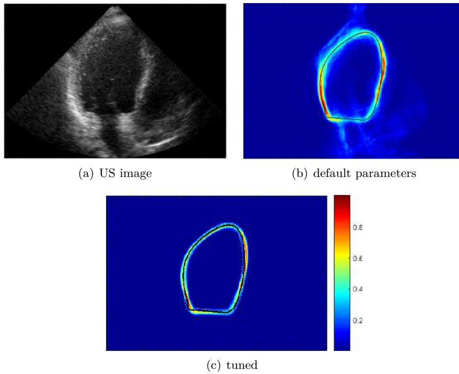
FIGURE 6.8: Detection of the endocardium using default or tuned SRF (multi-scale features + larger patch size + all trees used at test time).
