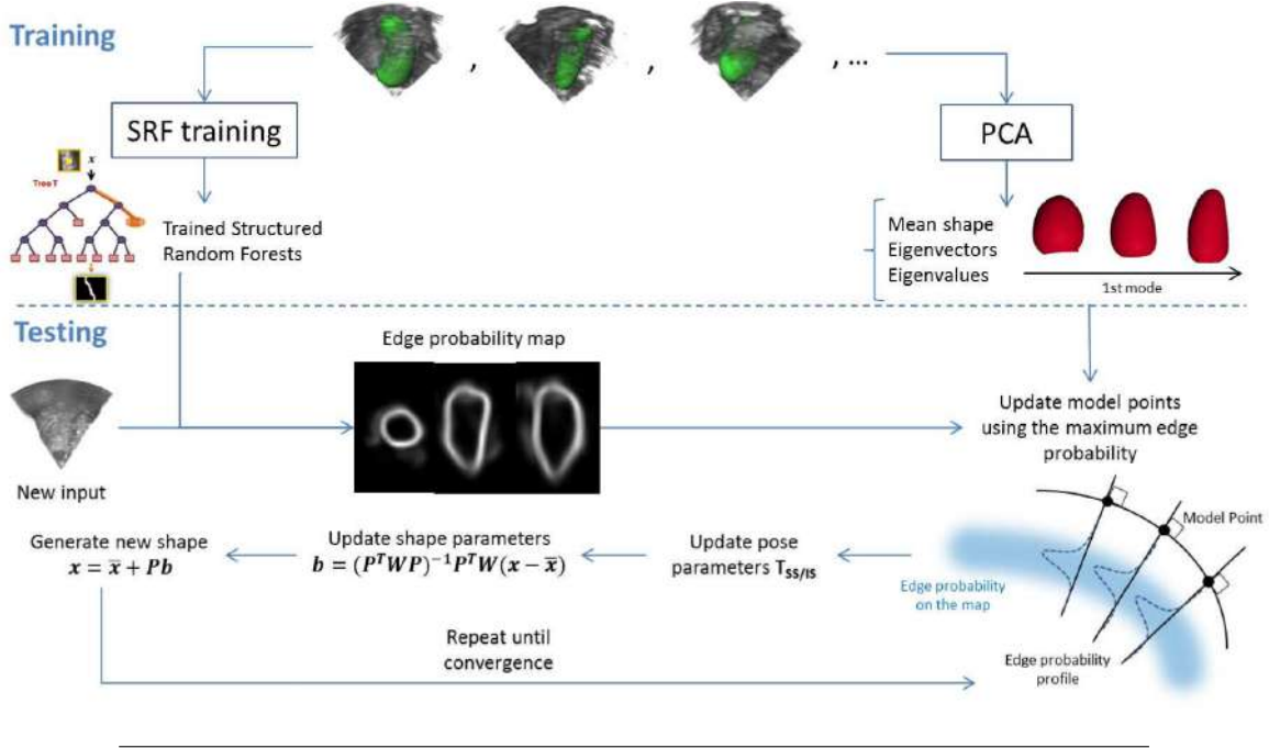
FIGURE 6.17: Overview of our complete pipeline combining SRF and ASM for 3D echocardiography segmentation.
