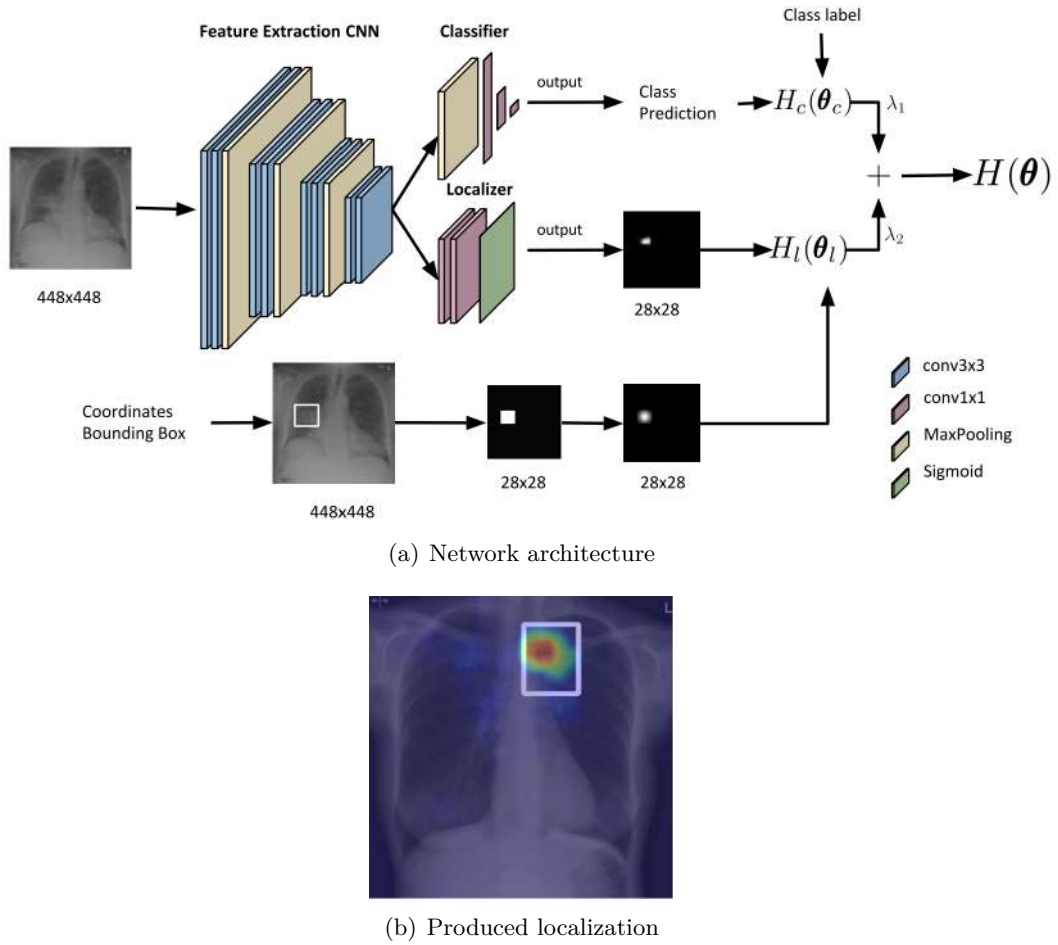
FIGURE 9.2: Pipeline and localization of lesion of (Pesce et al., 2019) [164].
