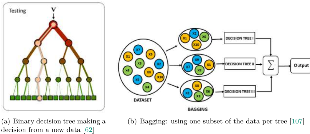
FIGURE 6.2: Core elements of the RF algorithm: binary decision tree (a) allied to randomizing strategies (such as b). Decision trees are a set of nodes routing the data to terminal nodes - called leaves - where the answer is stored.
