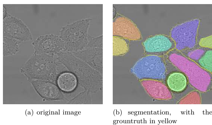
FIGURE 7.3: Example of cell segmentation with U-Net in microscopy images (DIC-HeLa data set) [34].
