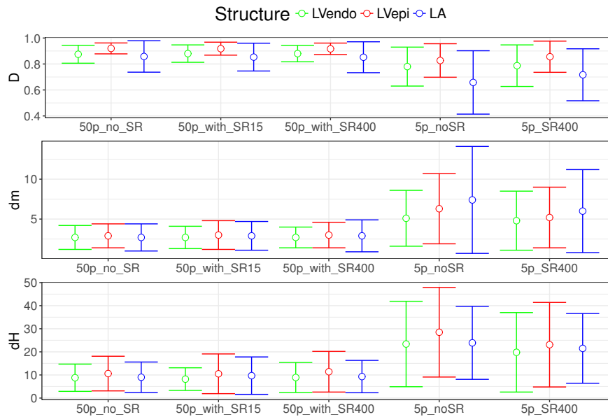
FIGURE F.2: Geometric performance of ACNNs illustrated by standard error bars around the mean values for the 5 segmentation networks.
