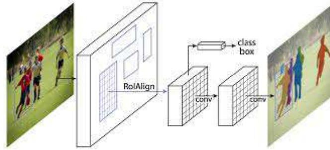
FIGURE 9.1: Mask R-CNN architecture of (He et al., 2017) [157]. A region proposal network isolates regions of interest that two parallel branches classify and segment.
