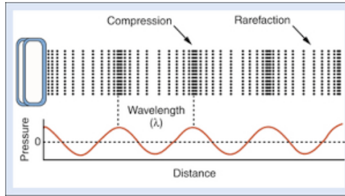
FIGURE 3.2: Longitudinal wave at a given time. As the wave propagates, particles oscillate between a compression or rarefaction state [8].
