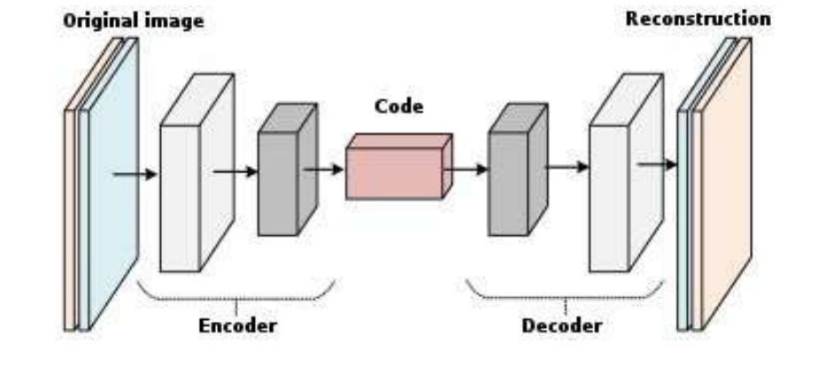
FIGURE 7.2: Auto-encoder architecture.
