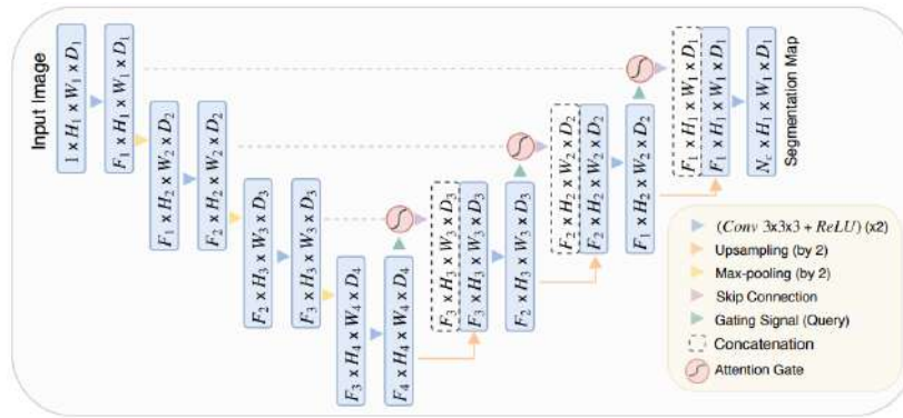
(a) AG-U-Net
