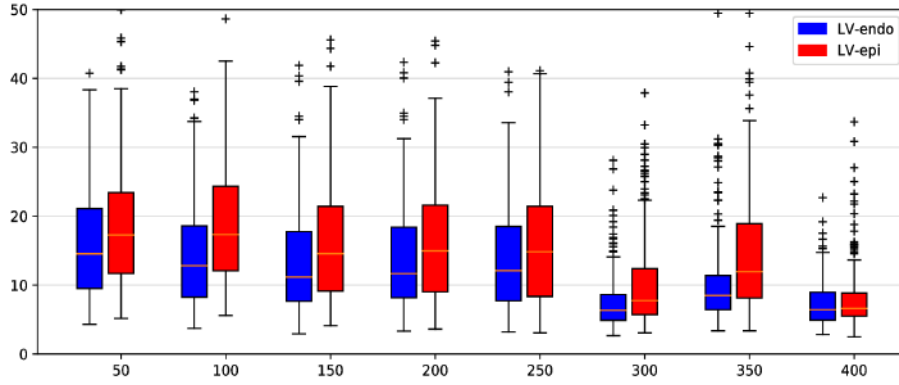
(a) Hausdorff distance (mm) evolution. The image is truncated at 50 mm for visibility.
