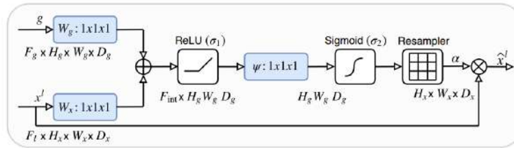
(b) soft attention layer
