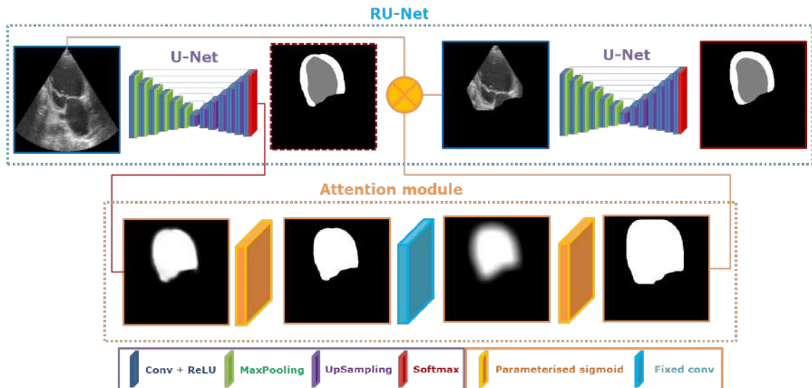
FIGURE 9.3: Illustration of the RU-Net pipeline. The two U-Nets are independent (different parameters).
