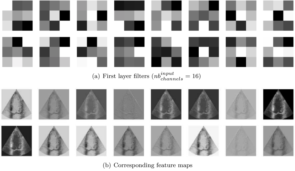
FIGURE 7.5: Visualization of the first layer filters learned by a reduced U-Net, and corresponding feature maps on a random validation image [122].
