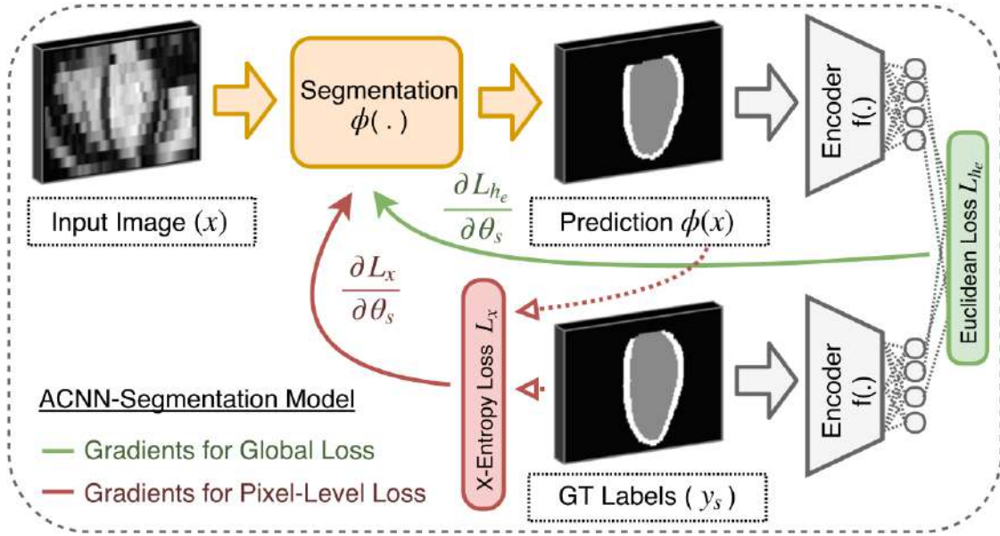
FIGURE 8.4: Pipeline for segmentation tasks of the ACNN model, introduced in (Oktay et al., 2017) [42].
