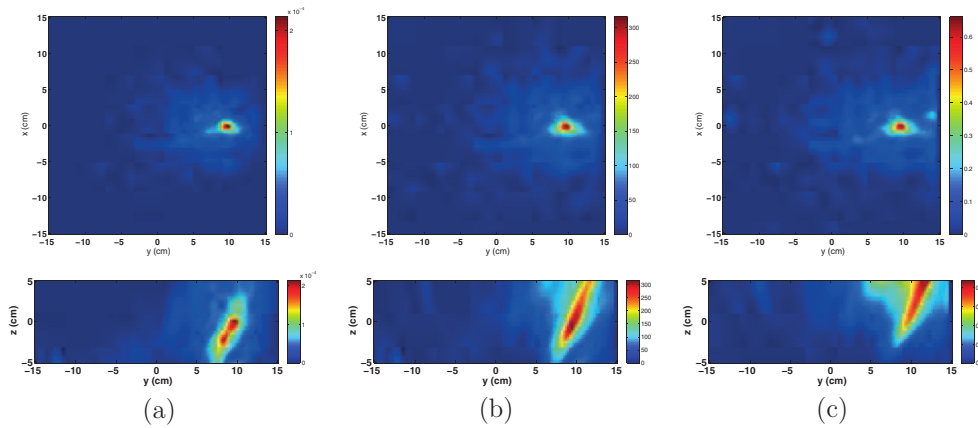
Figure 8. Point source placed in (0, 10, 0) cm emitting \gamma photons with energy of 5 MeV, reconstructed with different models of the sensitivity matrix. (a) MC sensitivity, (b) analytic sensitivity, (c) sensitivity set to 1.
