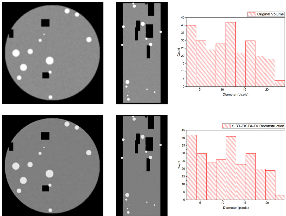
Fig. 3. SIRT-FISTA-TV reconstruction from complete and noiseless data. The first and second rows refer to original and reconstructed volume, respectively. Central cross-sections in XY- and XZ- planes are displayed in the first and second columns, respectively, and histograms for distribution of white inclusion diameters are shown in the third column.
