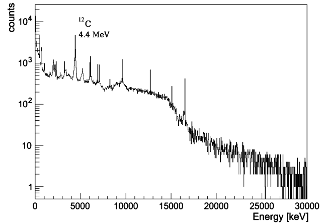
Fig. 3. Simulated energy spectrum of gamma rays with energies below 30 MeV leaving the PMMA phantom during irradiation by a proton beam at 140 MeV.
