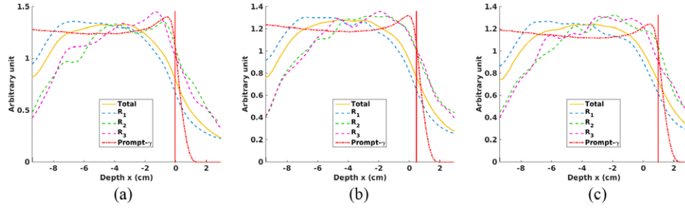
Figure 18. Overlay of the PG profile (dotted red line) and the reconstructed profiles calculated as projection of the central slice on 1 cm around the line y = 0 cm. The vertical red line stands for the PG fall-off. (a) [120 MeV] (b) [123 MeV] (c) [126 MeV].
