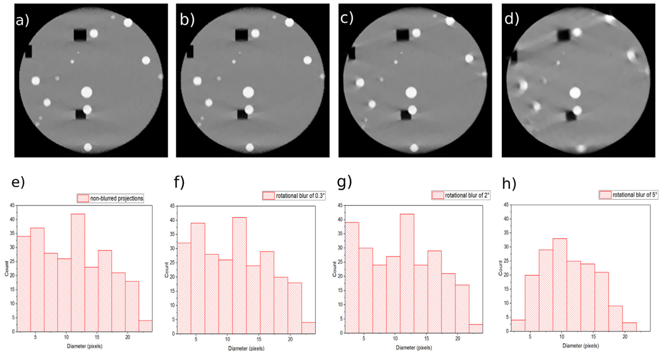
Fig. 10. SIRT-FISTA-TV reconstructions from non-blurred and blurred projections using a rotational blur of different degrees: 0.3°, 2° and 5°. (a): XY-plane cross-section in volume reconstructed with non-blurred projections. (b-d): XY-plane cross-sections in reconstructions with different degrees of rotational blur; (b) with 0.3°, (c) 2° and (d) 5°. (e): Histogram for distribution of white inclusion diameters within the volume reconstructed with non-blurred projections. (f-h): Histograms for distribution of white inclusion diameters within volumes reconstructed with different degrees of rotational blur; (f) with 0.3°, (g) 2° and (h) 5°.
