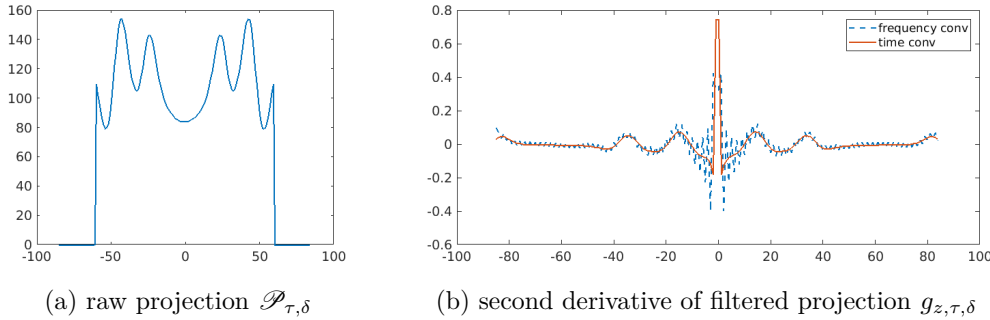
Figure 6: (a) Example of projection \mathcal{P}_{\tau,\delta} , i.e., Radon projection of the Compton projection, for a source composed of three points. (b) Its filtered versions g''_{z,\tau,\delta} for some arbitrary value z , with the convolution calculated in the frequency domain (blue dotted line) and in the time domain (red continuous line). The oscillations due to aliasing that may be observed in the right-hand image are important, but this is not always the case. Aliasing is more visible for large values of z\tau . Since they are attenuated by the usual smoothing of projections in the reconstruction process, the influence of the filtering domain may finally have little impact on the images.
