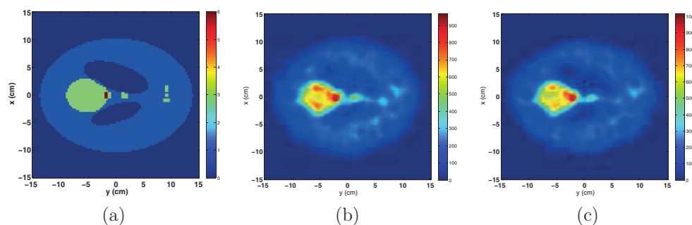
Figure 13. Two-dimensional Shepp–Logan phantom emitting at 662 keV, reconstructed in 3D with 40 iterations. The reference distribution is shown in (a). The reconstructed images are slices at z = 0 cm, corresponding to the position of the phantom. Realistic events without selection were considered for the reconstructed distribution shown in (b). A selection of the total energy deposited in the camera was operated for the image shown in (c).
