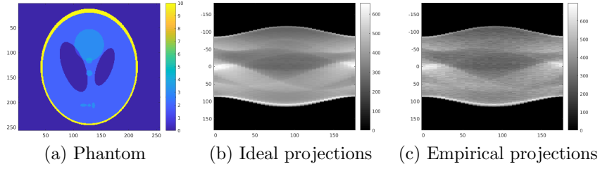
FIGURE 1. (a) Reference figure, the Shepp-Logan phantom and its sinograms: (b) without noise, (c) with Poisson random noise.
