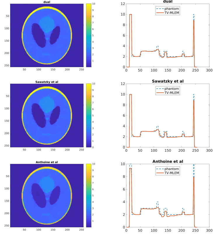
FIGURE 6. Comparison between the proposed dual method (first row), Sawatzky et al. (second row) and Anthoine et al. (third row) methods after 1000 MLEM iterations. We recall that the noise realization is different from figure 3 and thus the two figures should not be compared. The second column shows the central vertical profiles plotted along the images in the first column.
