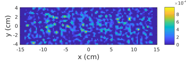
Figure 14: Low statistics reconstruction from ideal data, with the analytic formula.
