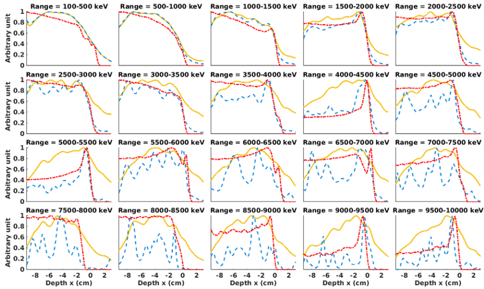
Figure 11. Overlay of three PG profiles: reference (dotted red line), reconstruction from events with total energy E_{\text{tot}} verifying |E_{\text{tot}} - E_0| \leq 250 keV (dashed blue line) and reconstruction from all the events (solid yellow line), for energy windows between 100 keV and 10 MeV with a 500 keV step. Projections calculated from the central slice on 1 cm around the line y = 0 cm.
