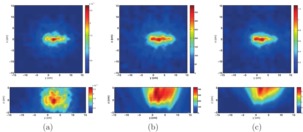
Figure 10. Images of a linear source with extremities (0, -2, 0) cm and (0, 10, 0) cm, emitting \gamma photons with energy of 5 MeV, reconstructed with different models of the sensitivity matrix. (a) MC sensitivity, (b) analytic sensitivity, (c) sensitivity set to 1.
