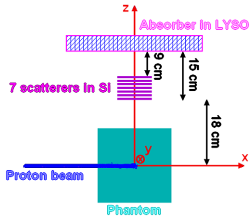
Figure 1. Simulation of the irradiation of a water phantom by a proton pencil beam with GATE. The distribution \lambda of the PG emission is extracted. The interaction of the PG photons in the Compton camera is simulated with MEGALib. The 3D distribution \hat{\lambda} is reconstructed with a LM-MLEM algorithm and projected on the central beam axis to obtain a 1D profile.
