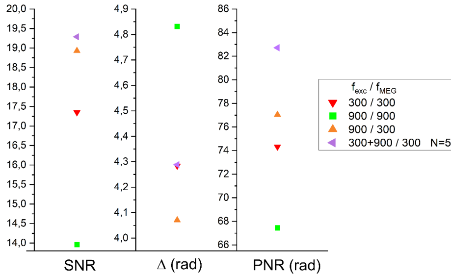
Figure 20. Plot of the SNR, \Delta and PNR values obtained with the different acquisition modes. SNR are in arbitrary unit, \Delta and PNR in radians. Note that each parameter has its own vertical axis. Only the acquisitions with trapezoidal MEGs are considered here. In the legend: conventional monofrequency acquisition ( \nabla, \square ), harmonic monofrequency acquisition ( \square ) and dual-frequency acquisition ( \triangleleft ) acquisition.
