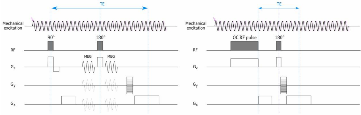
Figure 32. Sequence diagrams for the classical MRE (at left) and the OC-based MRE (at right) used in this study.
