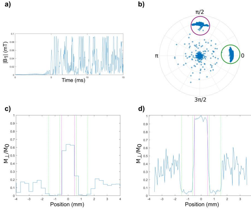
Figure 33. a) Temporal evolution of the magnitude of the OC RF pulse A ( B_1 = u_x ). b) Final transverse magnetization states in the Bloch sphere after the application of the OC pulse. The 0 (circled in green) and \pi/2 (circled in purple) phase isochromats are perfectly distinct. c). Simulated slice profile d) Experimental slice profile obtained with a RF profile sequence. The same resolution parameters were used in the simulation and experimental RF profile. The pink and green dashed lines in c and d represent the theoretical controlled slice thickness and outbands, respectively.
