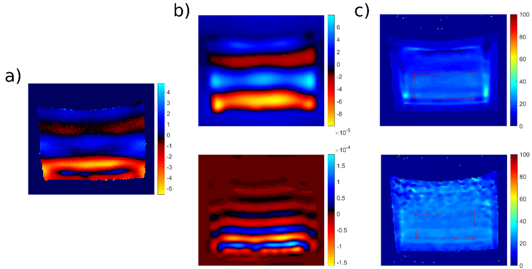
Figure 19. a) Phase image of the composite excitation (rad). b) Phase images (a.u.) and c) G' elastograms (kPa) of every extracted frequency component: 300 Hz on the top and 900 Hz on the bottom. ROI used for the computation of the shear storage modulus mean and standard deviations is showed in red lines on the cartographies of colon c.
