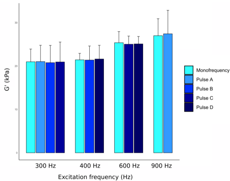
Figure 35. Mean values, with standard deviations displayed as error bars, of the reconstructed shear storage modulus G' for all the different excitation frequencies obtained with the classical monofrequency and the OC multifrequency methods.
