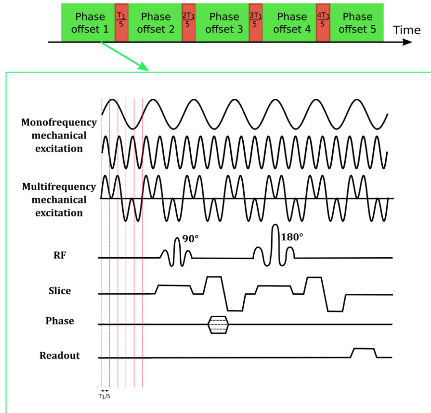
Figure 17. Chronogram of the multifrequency acquisition pulse sequence. The period of the lowest frequency mechanical vibration is denoted as T_1 . After the complete image of a phase offset has been acquired (green square), a delay of T_1/5 (red square) is added to perform the acquisition for the next phase offset image.
