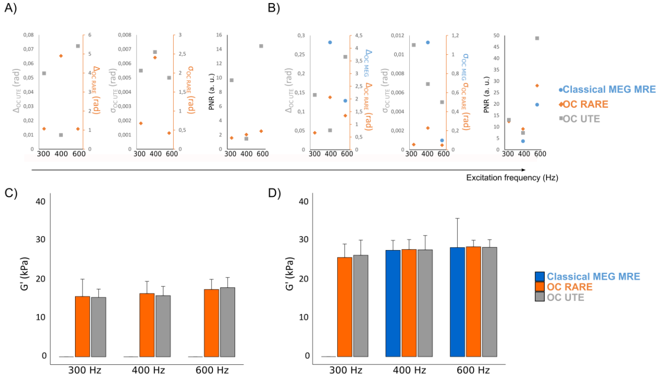
Figure 29. Results of phase encoding \Delta , phase noise \sigma and Phase-to-Noise ratio PNR obtained with the different acquisitions at multiple frequencies on the A) 5 mM and the B) 1 mM \text{MnCl}_2 concentration layers. Note that two vertical axis are showed in phase encoding and phase noise plots. Mean values and standard deviation of the shear storage modulus G' obtained for all the excitations frequencies with the different sequences on the C) 5 mM and the D) 1 mM \text{MnCl}_2 concentration layers.
