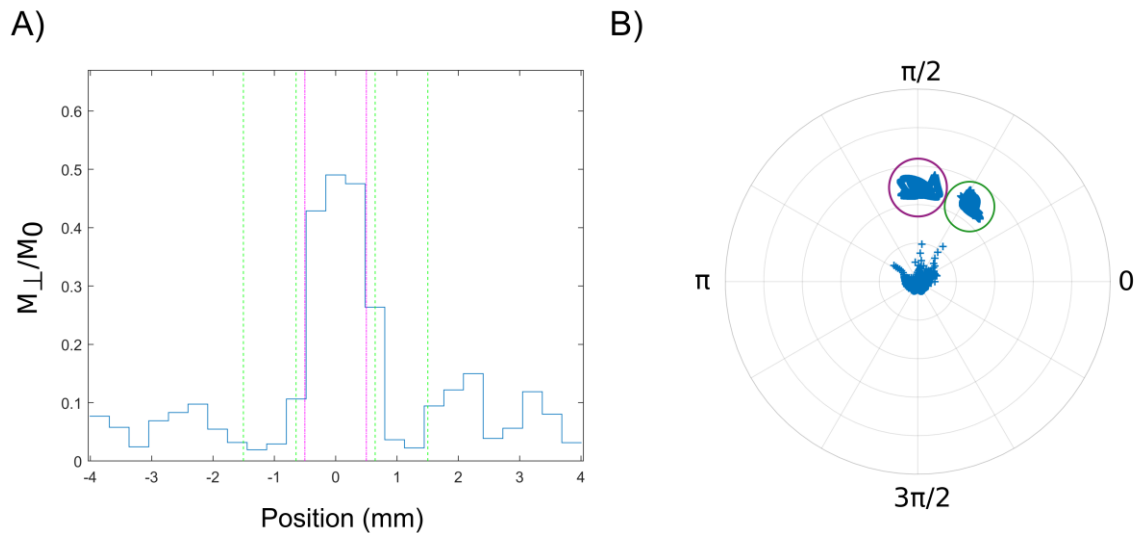
Figure 26. Characteristics of the OC pulse C: A) Simulated slice profile. The pink and green dashed lines represent the theoretical controlled slice thickness and outbands, respectively. B) Final transverse magnetization states in the Bloch sphere after the application of the OC pulse. The 0 (circled in green) and \pi/2 (circled in purple) isochromats are perfectly distinct. The groupe in the center represents the isochromats outside the bandwidth.
