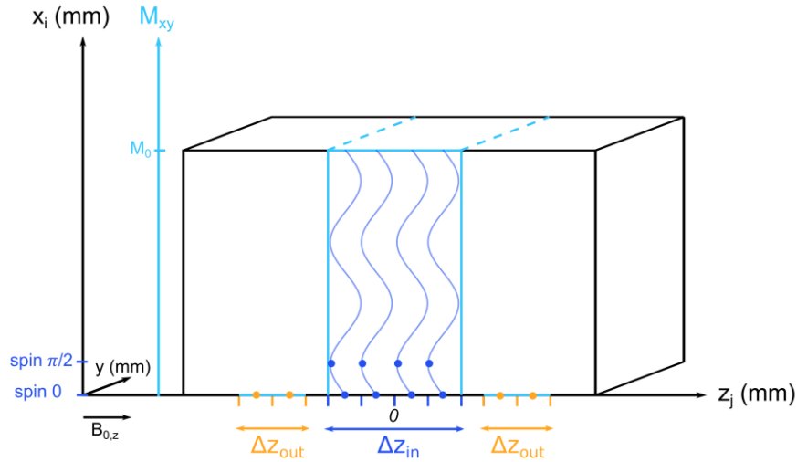
Figure 25. Definition of the numerical phantom to solve the OC problem applied to MRE. Motion of spins induced by the shear wave is represented in dark blue oscillations. Note that two different vertical axes are considered.
