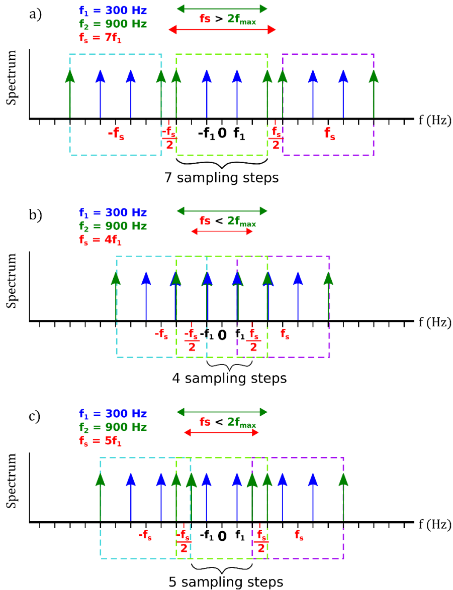
Figure 16. Different representations of the spectra obtained in the frequency domain after temporal Fourier Transform of sampled points at a sampling frequency f_s . The original signal was a dual-
