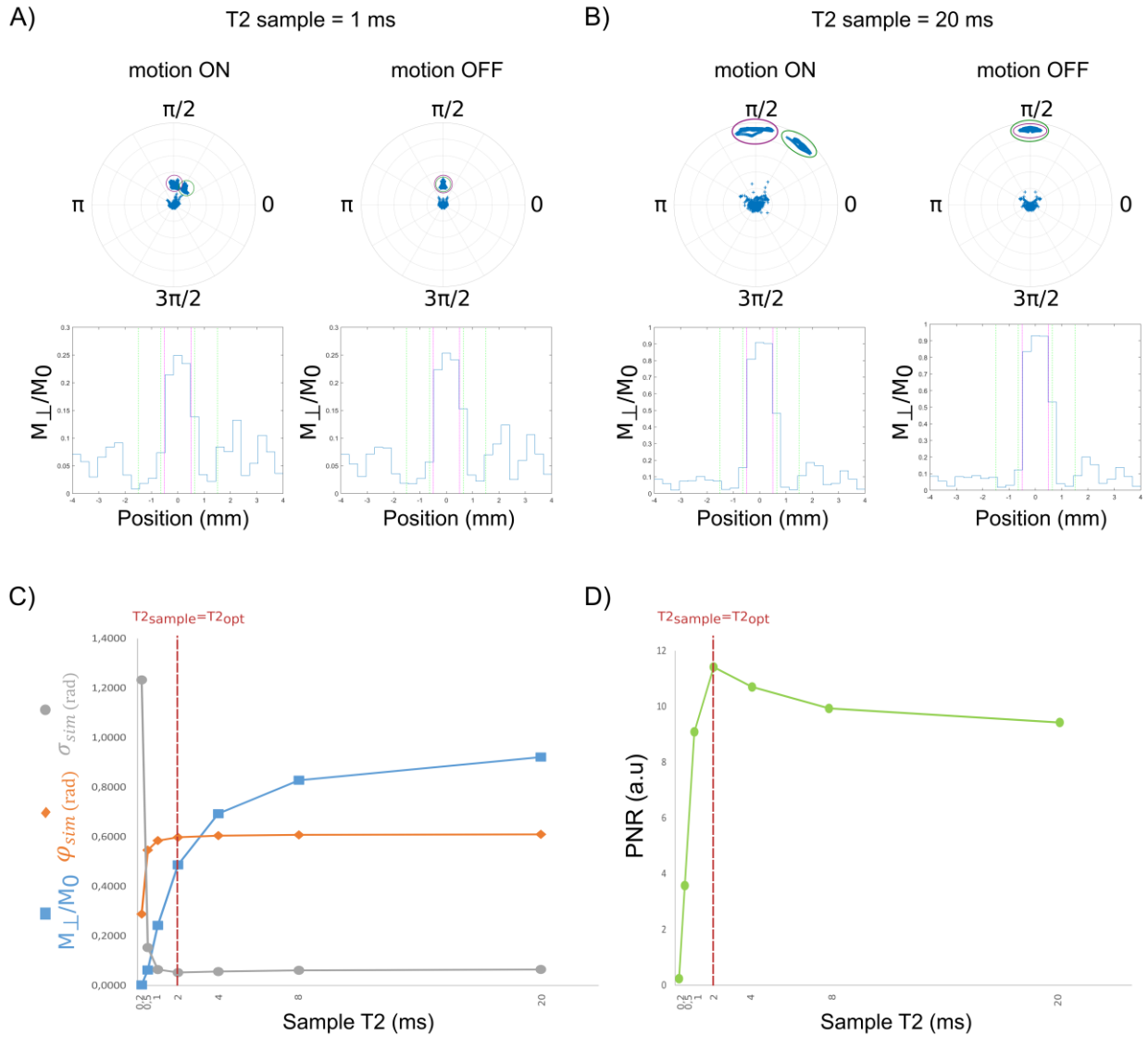
Figure 27. Numerical evaluation of the robustness of the OC pulse C with respect to the variability of the sample T_2 . Final transverse magnetization states in the transverse plane after the application of the OC pulse and simulated slice profiles with and without motion for samples with T_2 values of : A) 1 ms B) 20 ms. C) Simulated encoded phase, phase noise, transverse magnetization amplitude and D) PNR variation with respect to the sample T_2 which varies between 0.2 and 20 ms.
