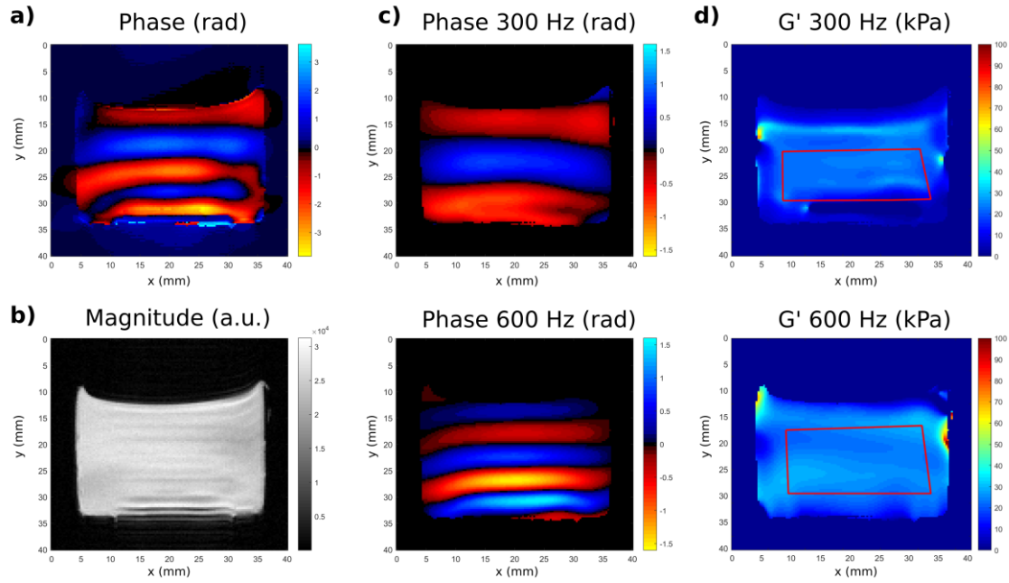
Figure 34. a) Phase and b) magnitude images of the composite excitation 300 Hz and 600 Hz acquired with the OC pulse C. c) Then separated in phase images (rad) of every frequency component extracted after temporal Fourier transform, choice of the corresponding harmonics and application of the inverse Fourier transform: top: 300 Hz; bottom: 600Hz. d) G' elastograms (kPa) reconstructed for each frequency component: top: 300 Hz; bottom: 600Hz. The ROIs used for the computation of the shear storage modulus mean and standard deviations are shown with red lines on the maps in c.
