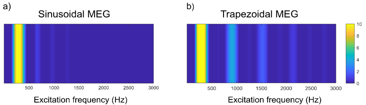
Figure 15. Accumulated phase with one cycle of 300 Hz MEG for different excitation frequencies and with various oscillating gradient shapes. Left: sinusoidal-shaped; Right: trapezoidal-shaped. Values are in arbitrary units and were scaled from 0 to 10 for a better visualization. The periodical behavior of the sensitivity bands is visible when using a trapezoidal MEG.
