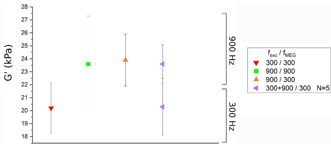
Figure 21. Mean values, with standard errors displayed as error bars, of the reconstructed shear storage modulus G' for both excitation frequencies (300 and 900 Hz) obtained with the different acquisition modes. Only the acquisitions with trapezoidal MEGs are considered here. An excellent agreement of the G' values is found for all the cases.
