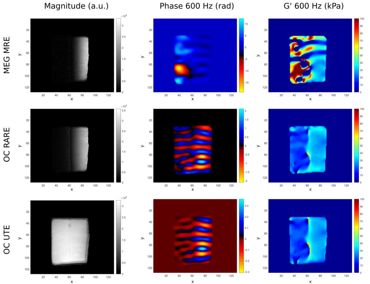
Figure 28. Magnitude, phase and shear storage modulus G' images obtained at 600 Hz with the different sequences : classical MEG MRE, OC RARE and OC UTE. For the OC sequences, pulse C was used.
