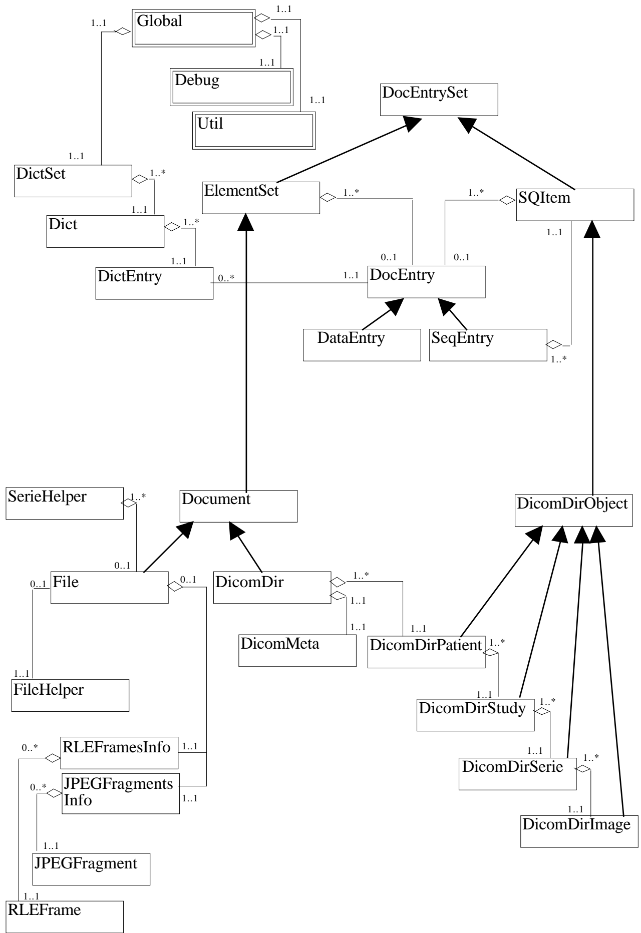
gdcm UML Classes Diagram
